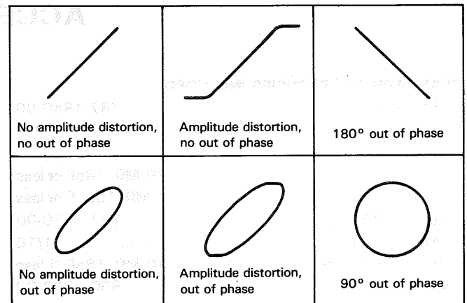
Fig. 43 Typical phase measurement oscilloscope display
